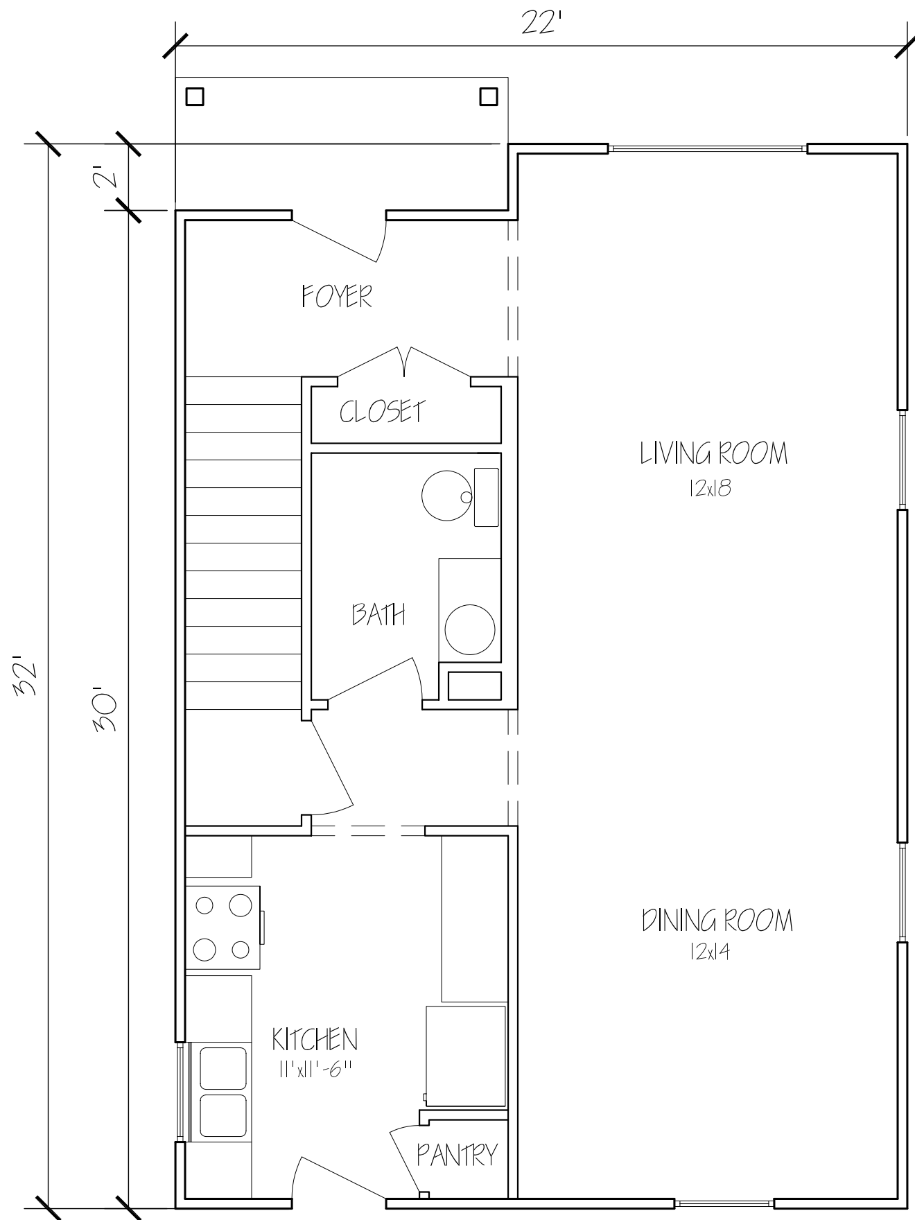
FIRST FLOOR PLAN 684 SF
