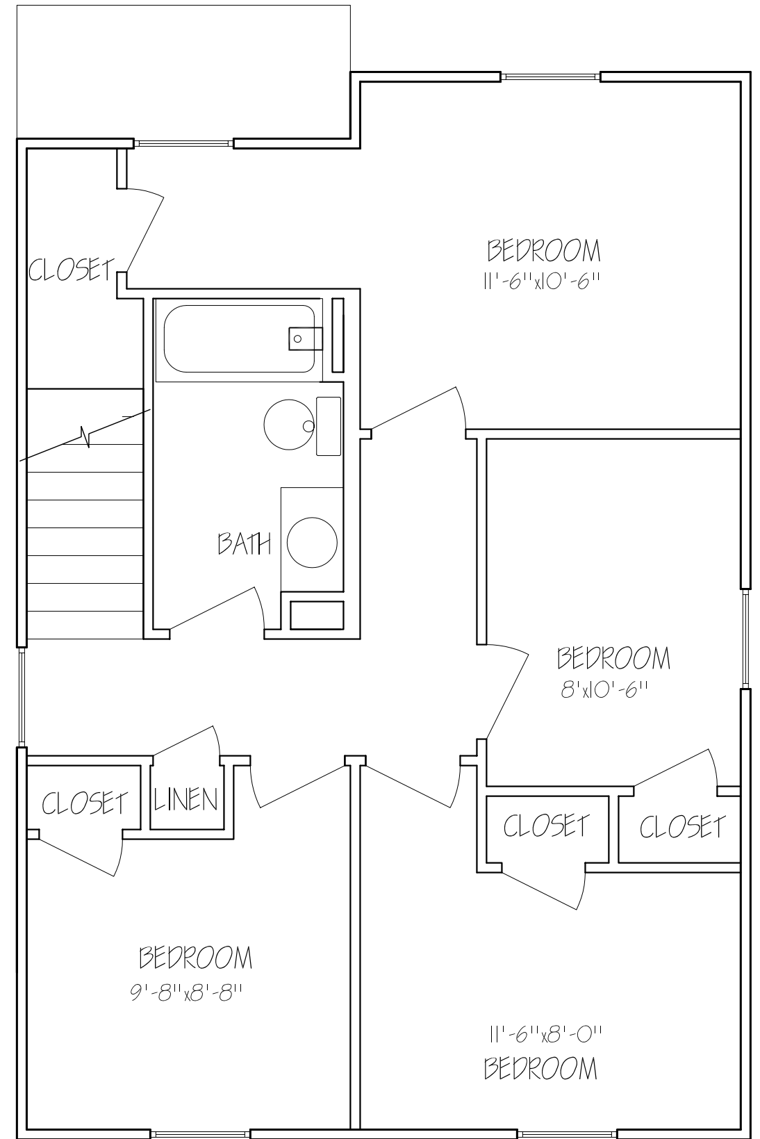
SECOND FLOOR PLAN 684 SF
